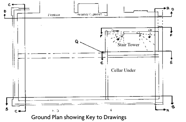
Ground Plan showing key to Drawings
